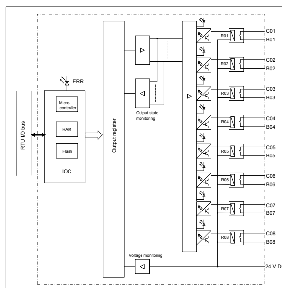
Figure 1: Block diagram 520BOD01
