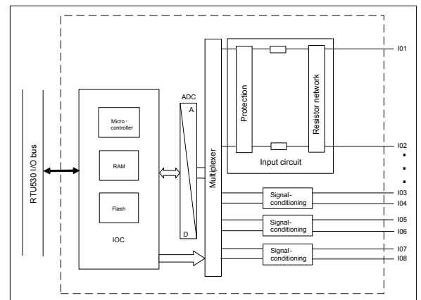
Figure 1: Block diagram 530AID01
