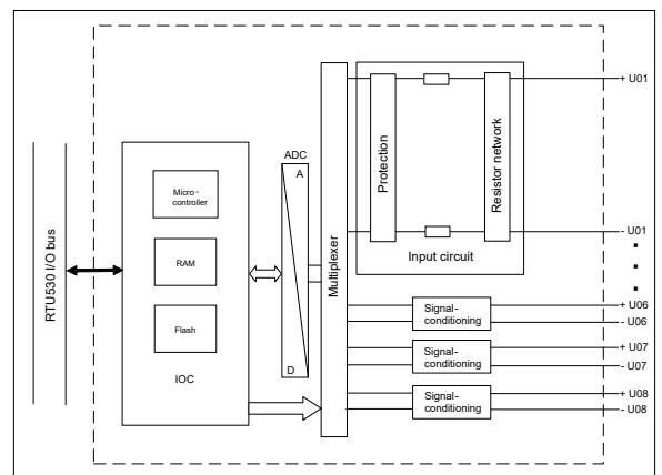
Figure 1: Block diagram 530AID02
