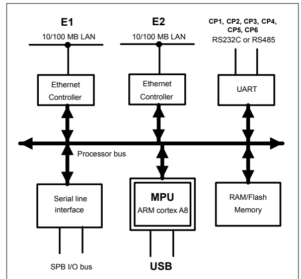
Figure 1: Block diagram 560CMR02
